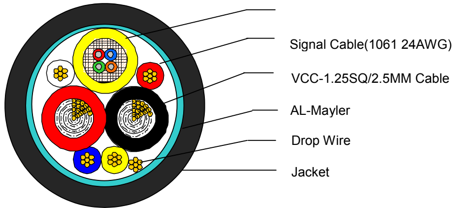
Figure 1. Cable structure of HDMB2
